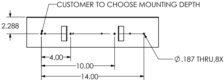
SSG 1.5K RM MOUNTING HOLE PATTERN
